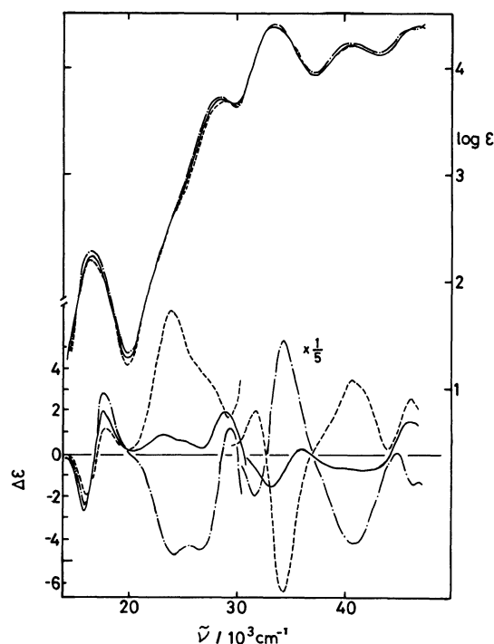
Fig. 3. Absorption and CD spectra of trans -[CoCl 2 ( RS(P) - SS(C) -mp-PNNP)] + (—), trans -[CoCl 2 ( SS(P) - SS(C) -mp-PNNP)] + (---), and trans -[CoCl 2 ( RR(P) - SS(C) -mp-PNNP)] + (-·-·-).
